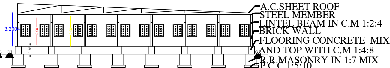
SECTION ON A-A
