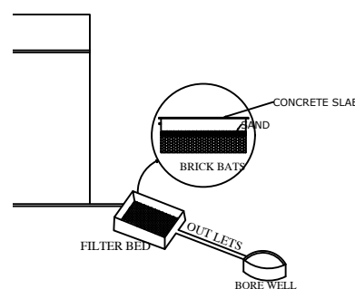
WATER HARVESTING TANK
