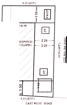
PLAN ( SCALE 1:100 )
