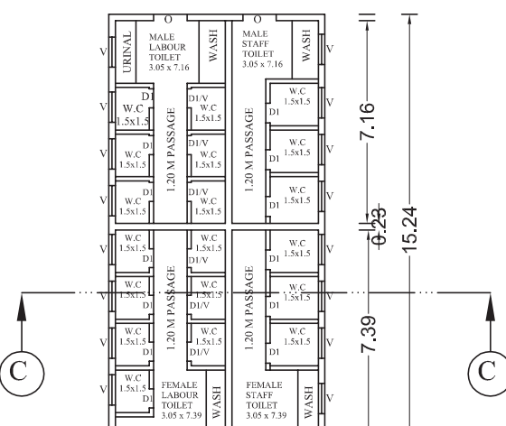
BLOCK - 3- GROUND FLOOR - TOILET BLOCK BUILDING
