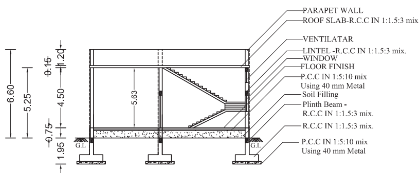
SECTION OF B-B
