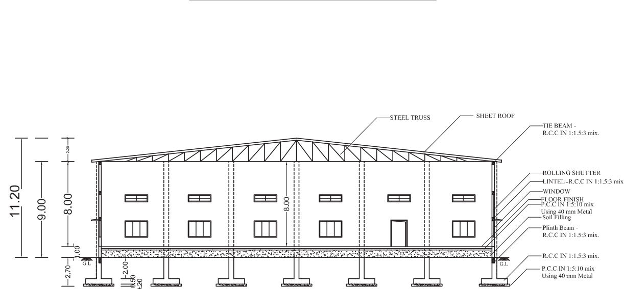
ELEVATION FACING NORTHSIDE
