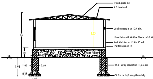
Section on "BC"
