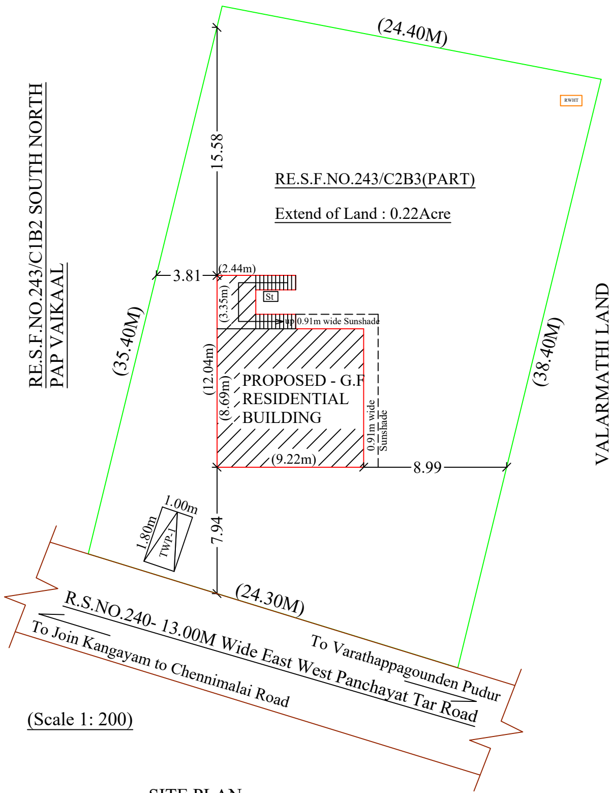
SITE PLAN
