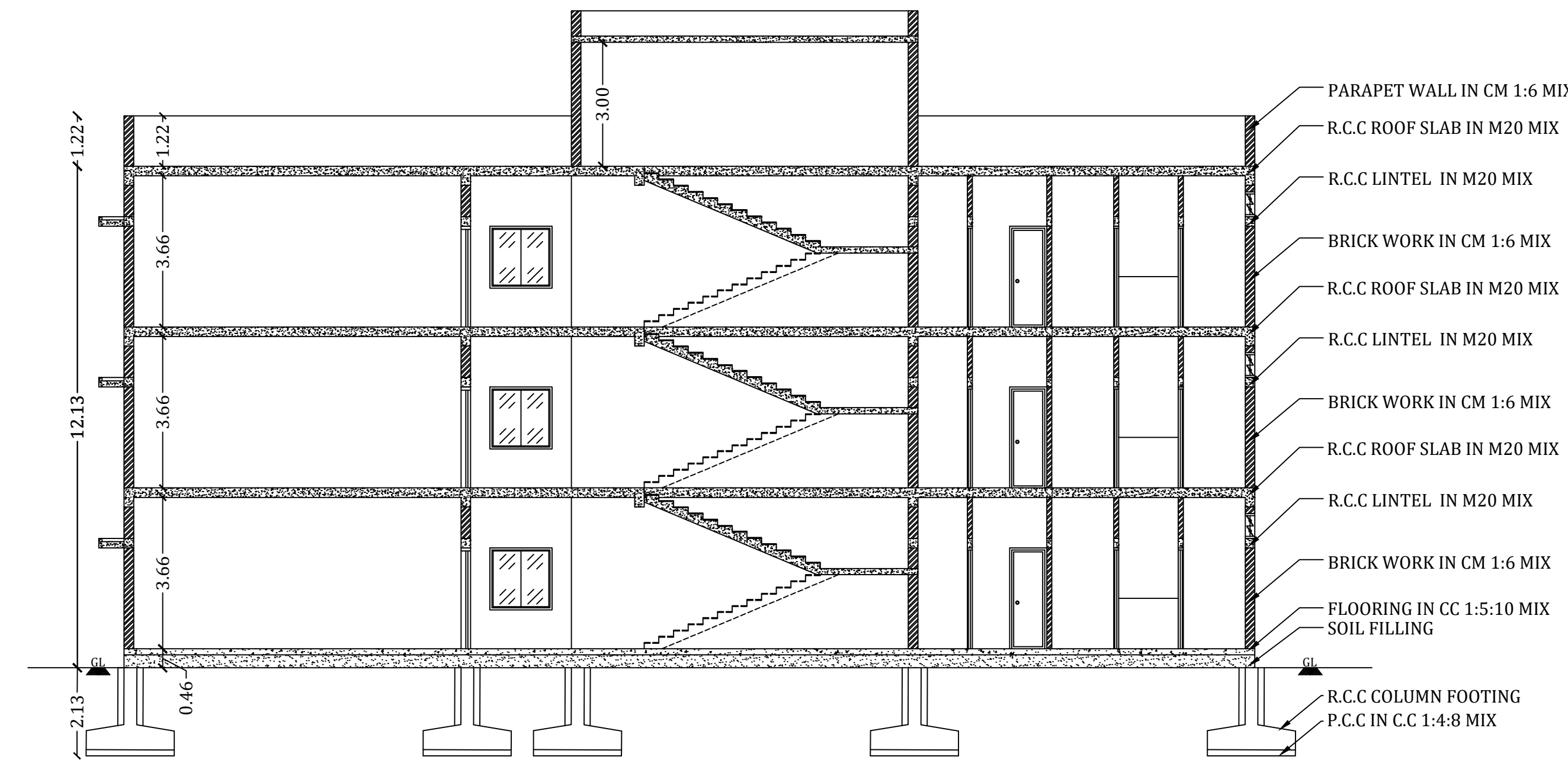
SECTION OF A-A SCALE = 1:100
