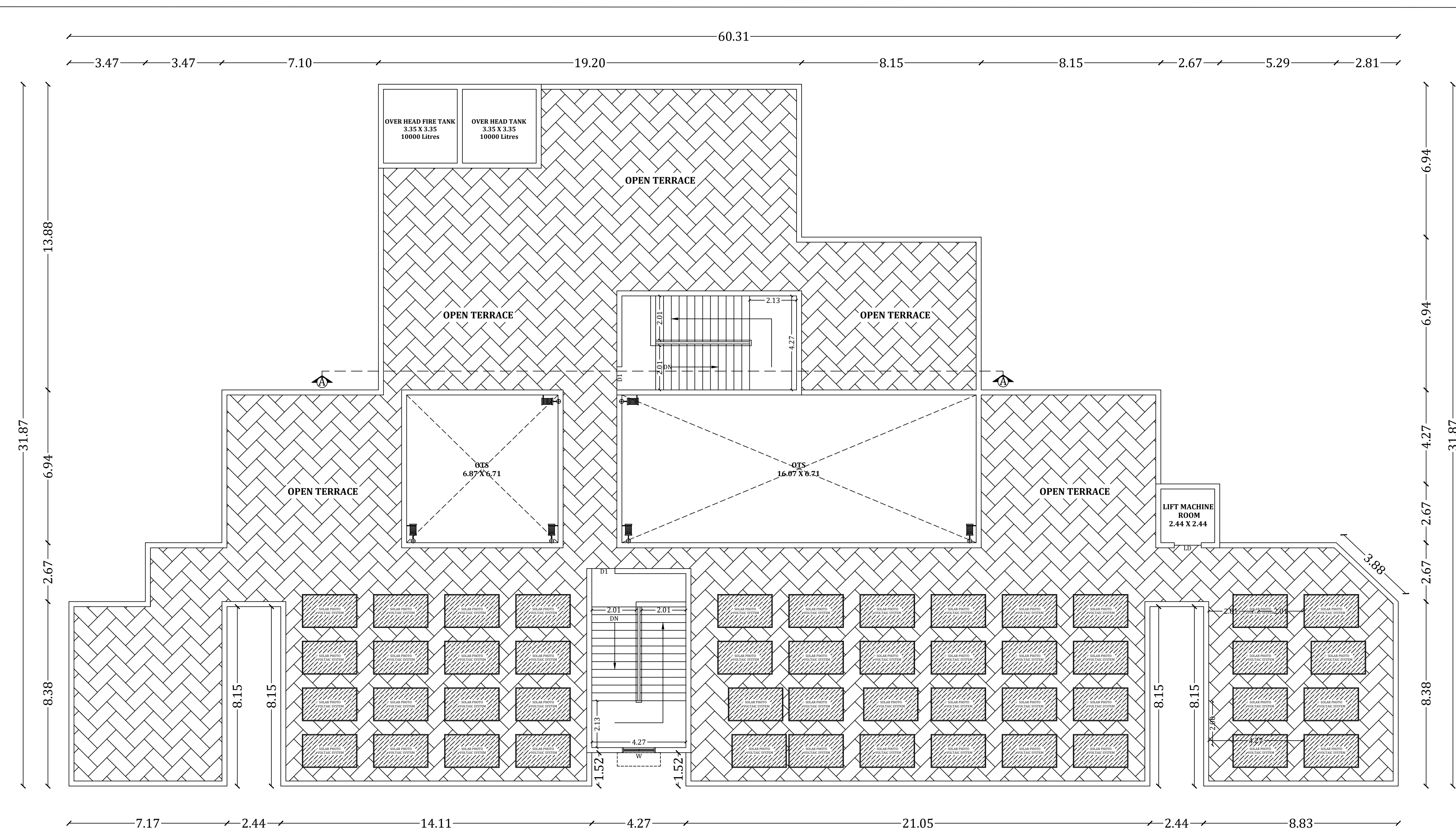
TERRACE FLOOR PLAN SCALE = 1:100
