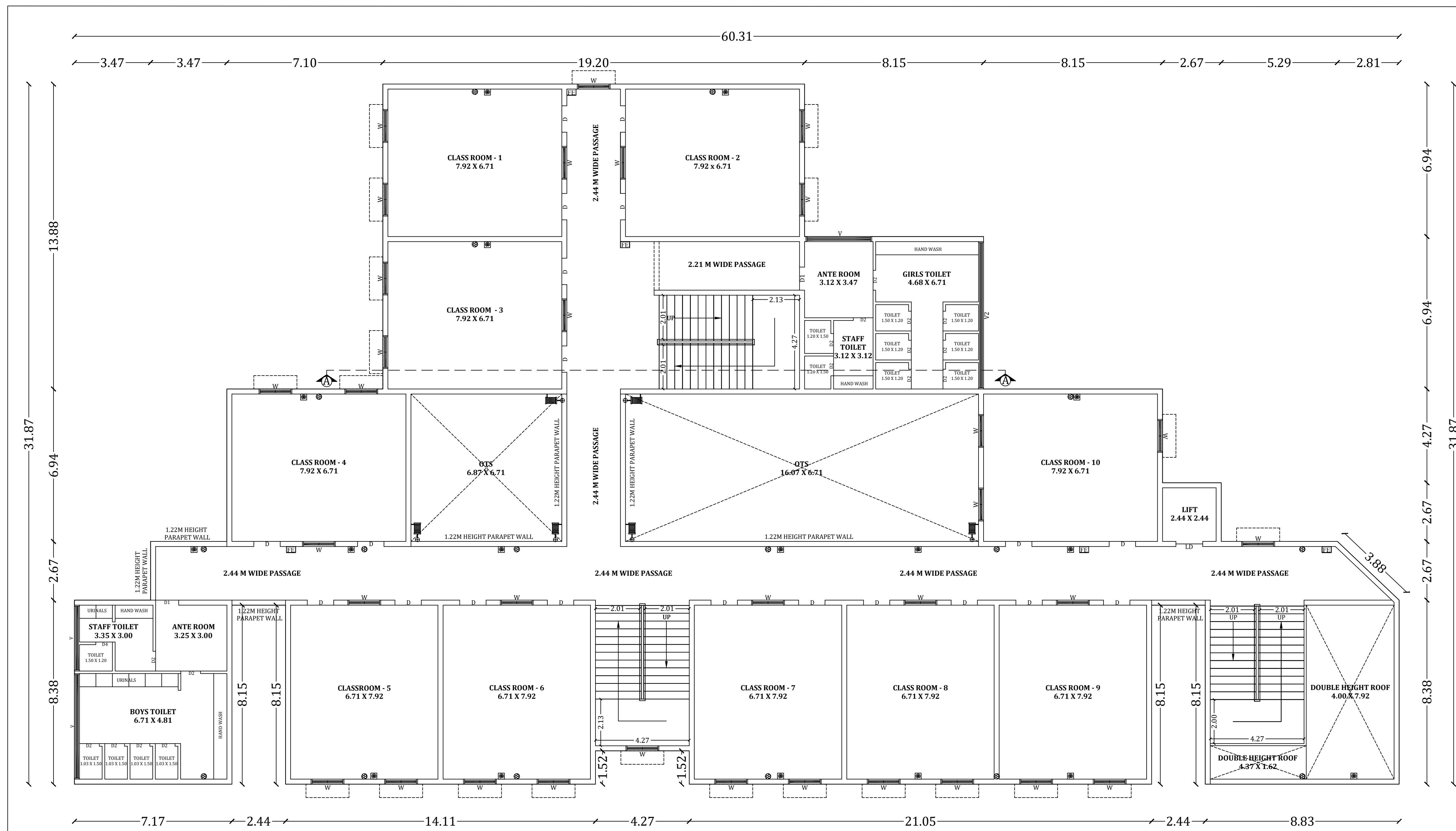
FIRST FLOOR PLAN SCALE = 1:100
