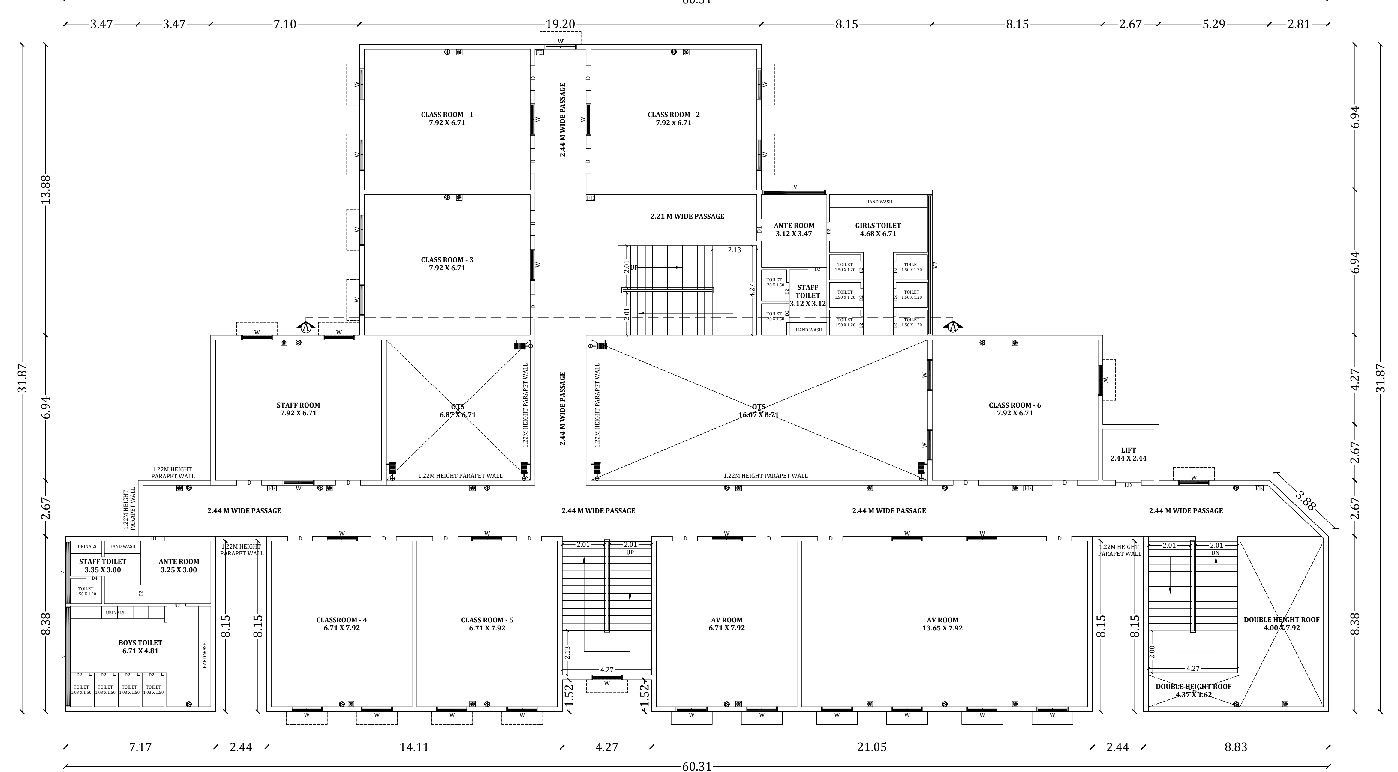
SECOND FLOOR PLAN SCALE = 1:100
