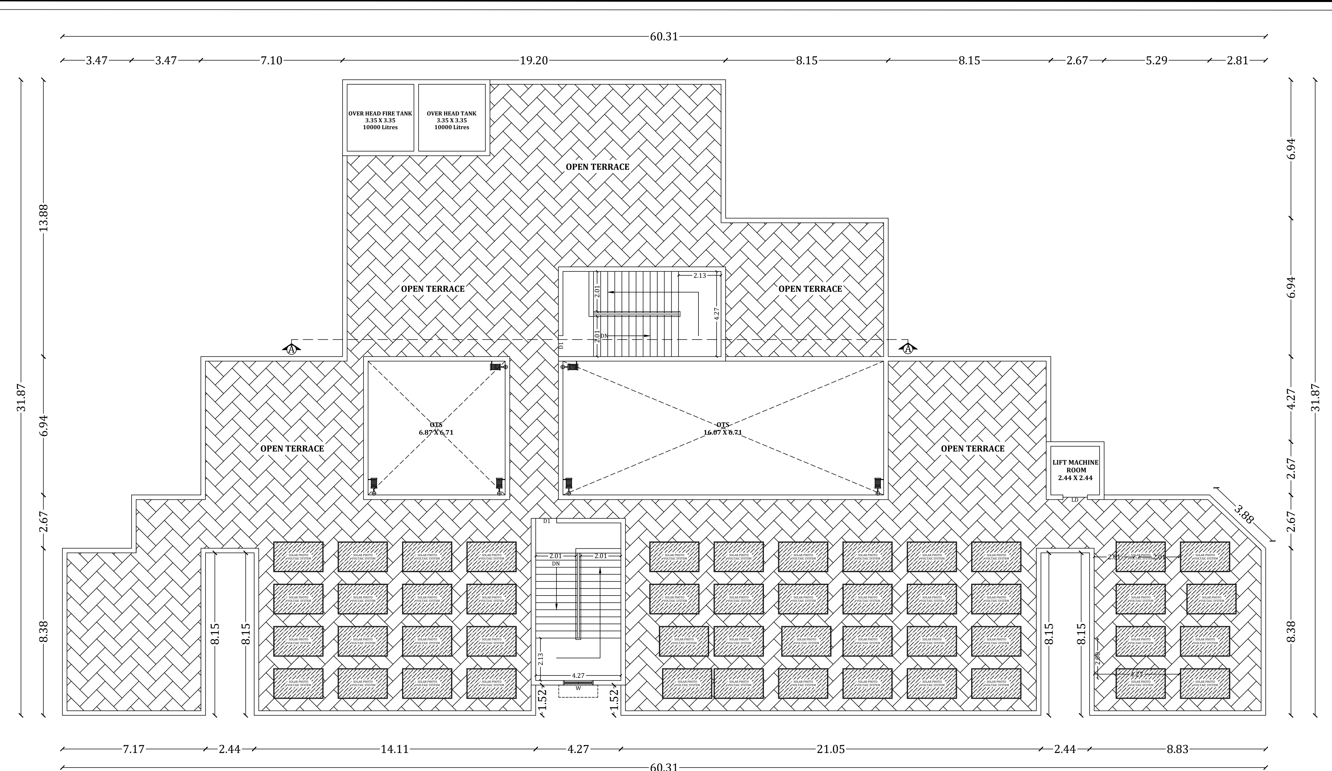
TERRACE FLOOR PLAN SCALE = 1:100
