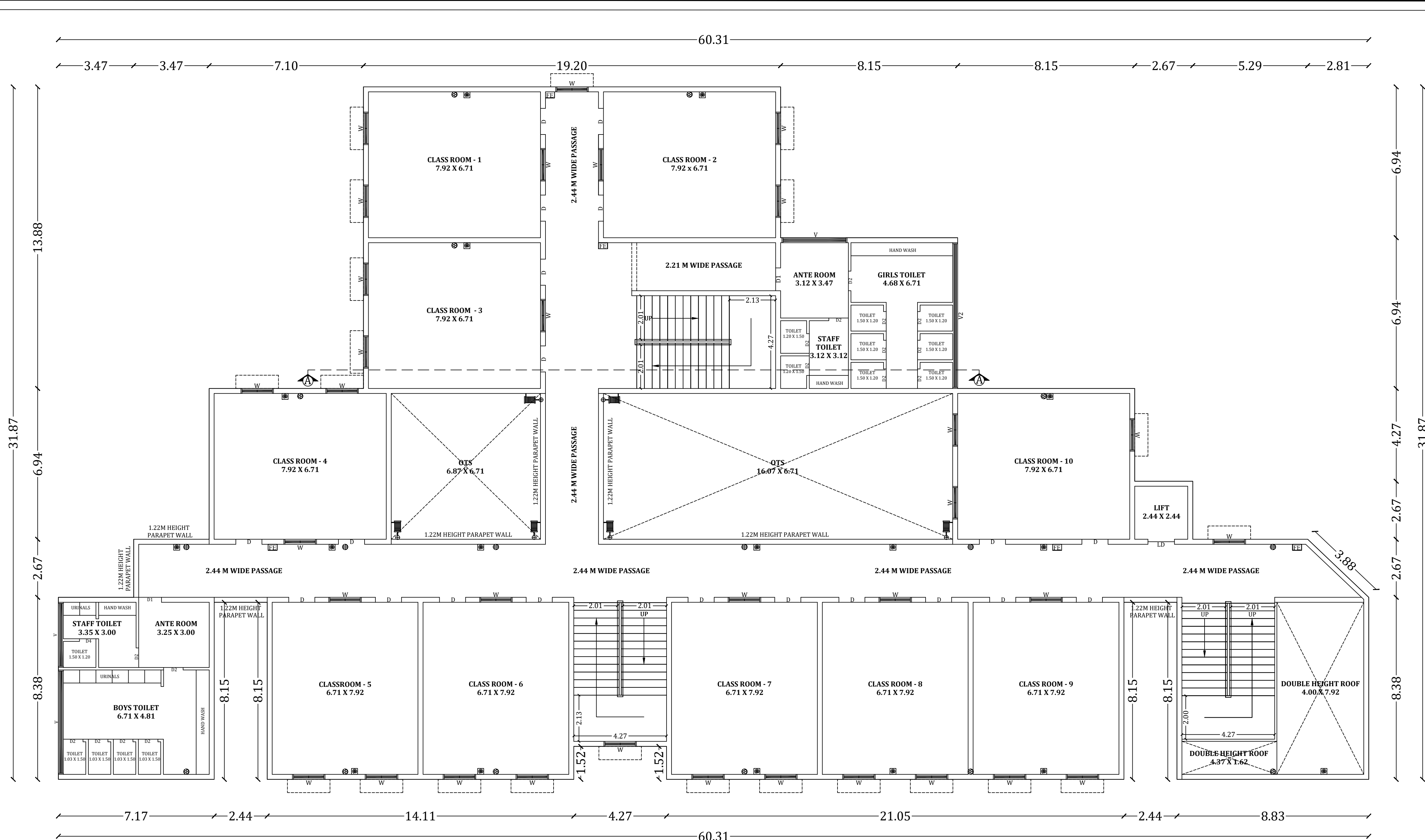
FIRST FLOOR PLAN SCALE = 1:100
