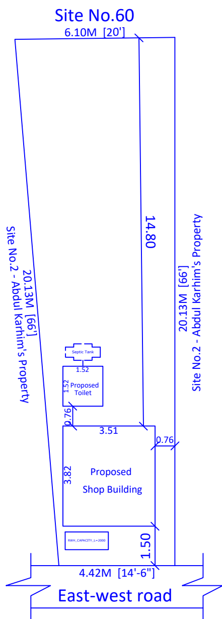
SITE PLAN
