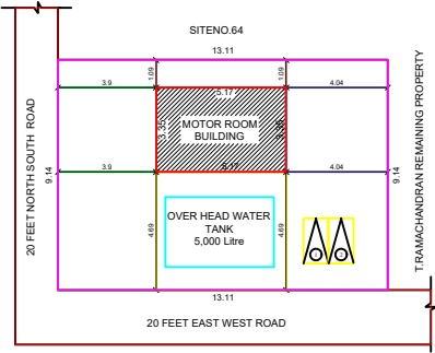
SITE PLAN
