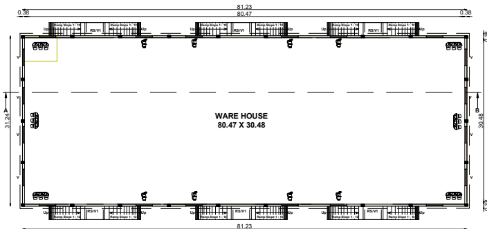
WARE HOUSE GROUND FLOOR PLAN (BLOCK -1)
