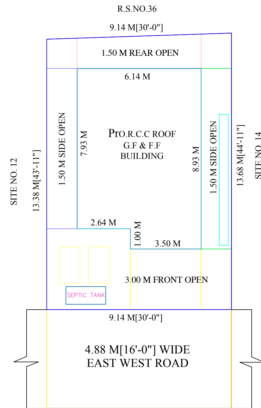
SITE PLAN
