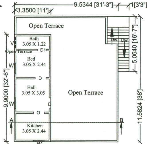
PRO. FIRST FLOOR RESIDENTIAL BLDG. PLAN
