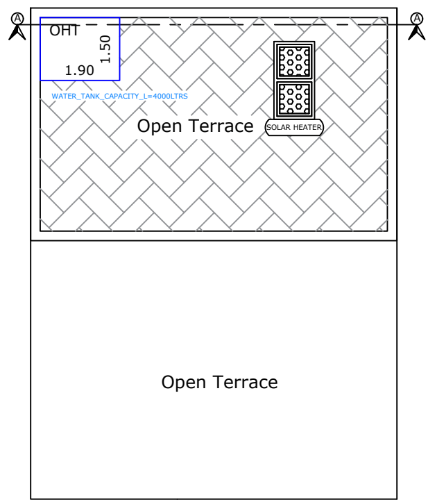
PROPOSED TERRACE FLOOR PLAN
