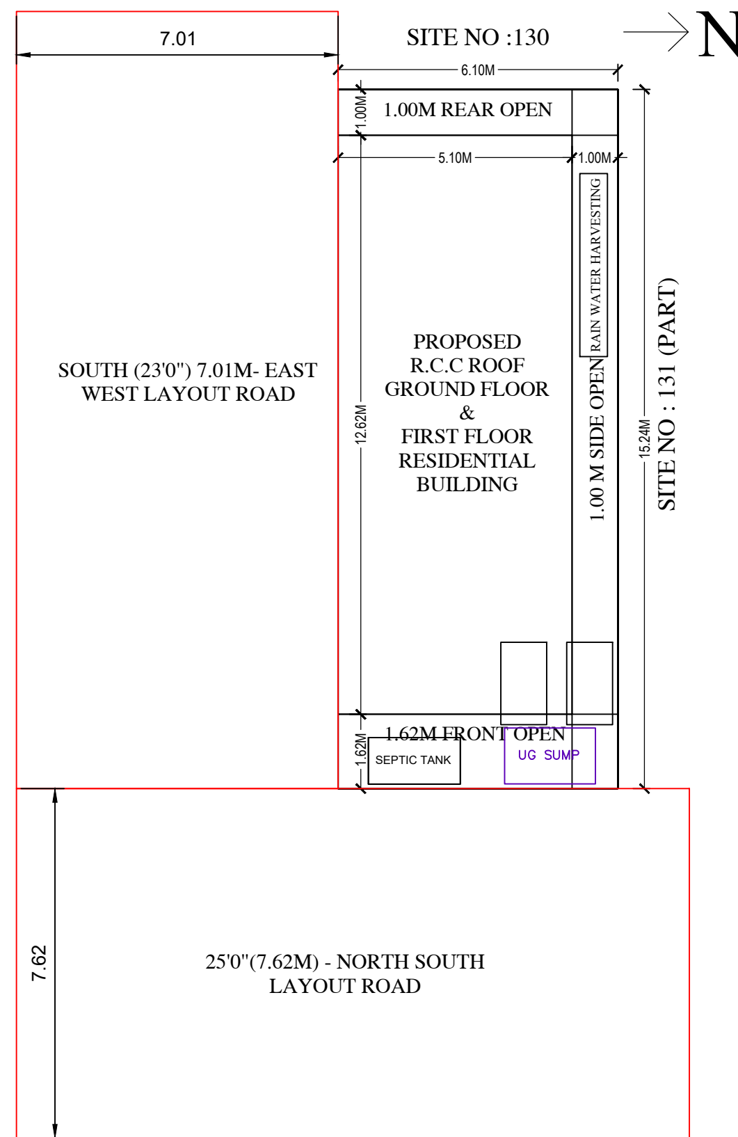
SITE PLAN
