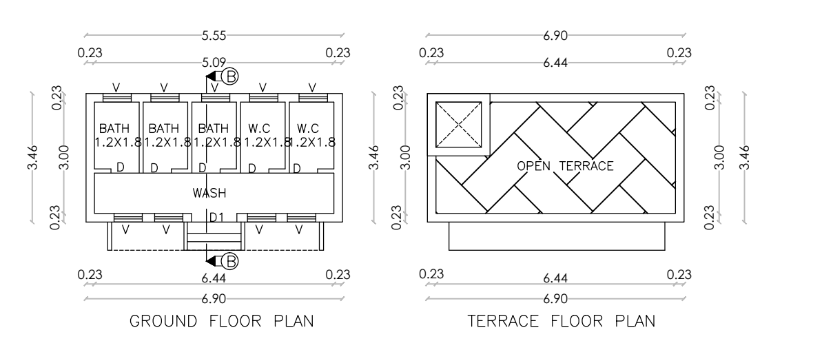
PRO.TOILET BLOCK
