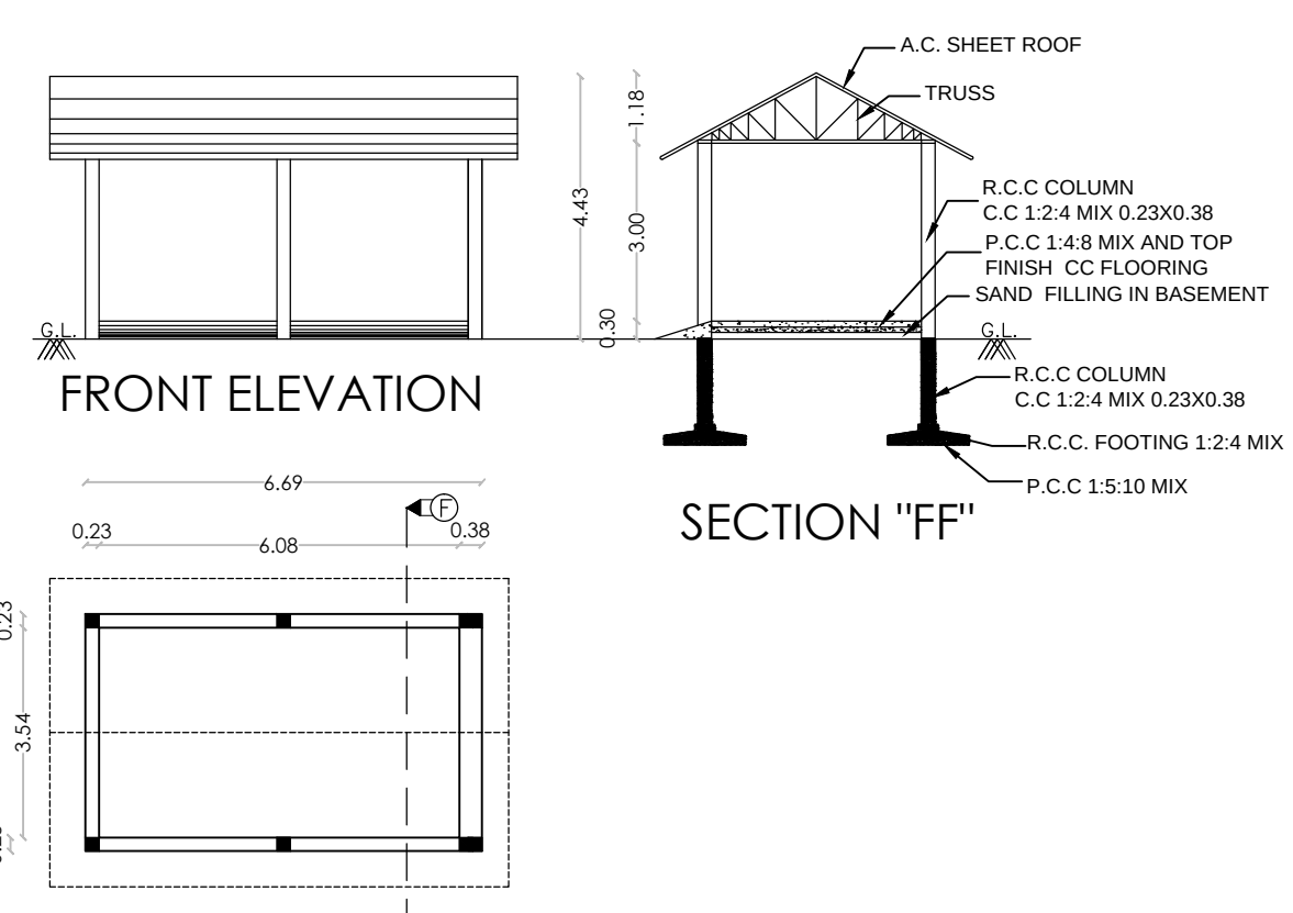
GROUND FLOOR PLAN PRO.FUNERAL VAN SHED
