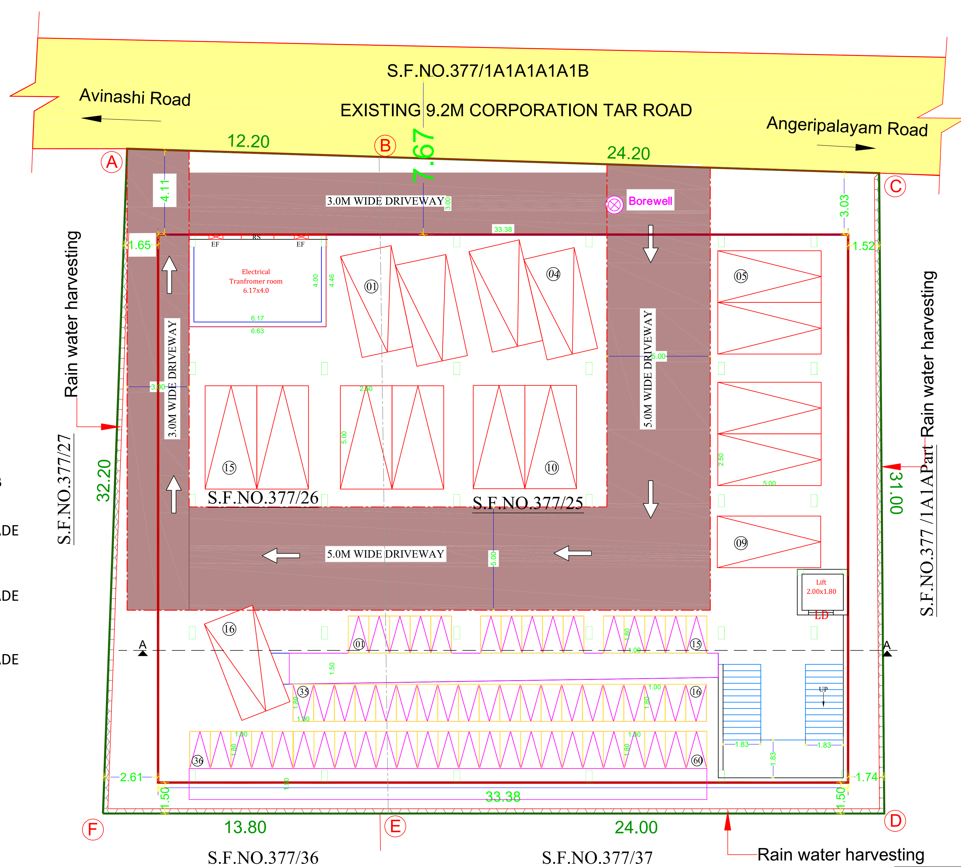
SITE CUM STILT FLOOR PLAN
