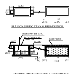
SECTION ON SEPTIC TANK & DISP-TRENCH
