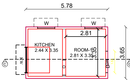
GROUND FLOOR PLAN BLOCK -2 SCALE (1:100)
