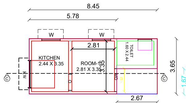
GROUND FLOOR PLAN BLOCK -2 SCALE (1:100)
