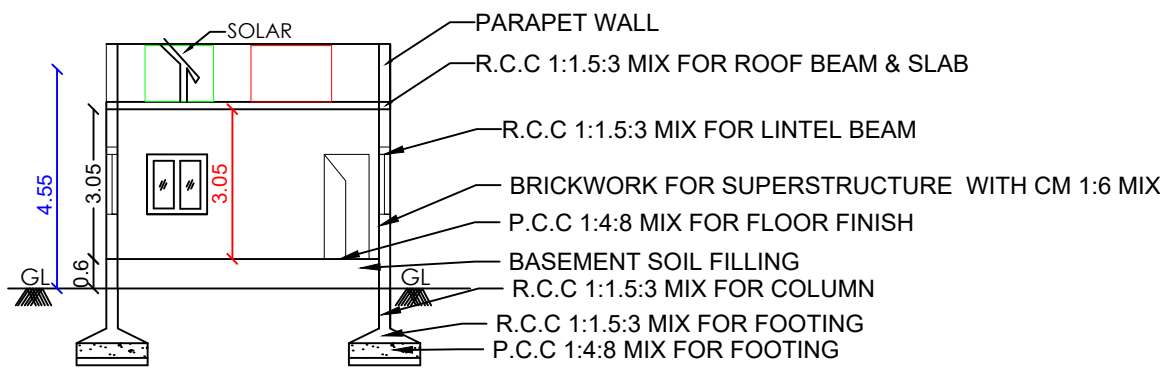
SECTION ON B-B
