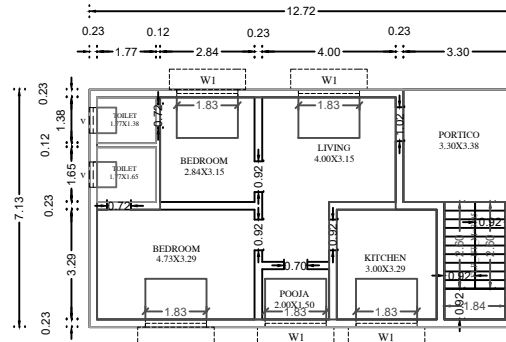
PRO.GROUND FLOOR PLAN
