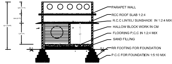
SECTION ON-AA
