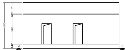
ELEVATION FACING EAST
