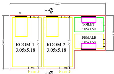
GROUND FLOOR
