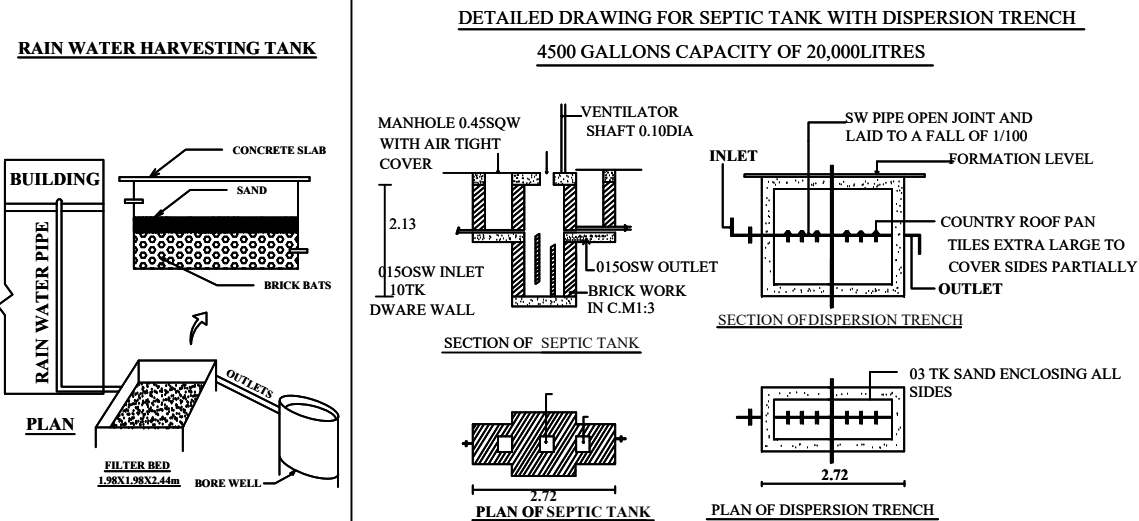
JOINARY DETAILS
