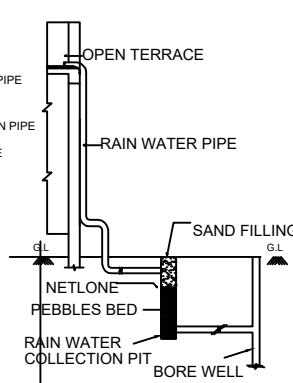
RAIN WATER
