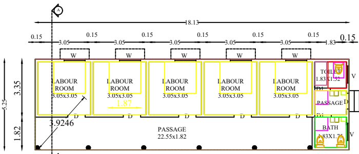
LABOUR SHED BLOCK - 1
