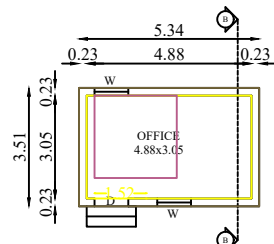
OFFICE PLAN BLOCK - 2
