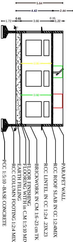
SECTION ON A-A
