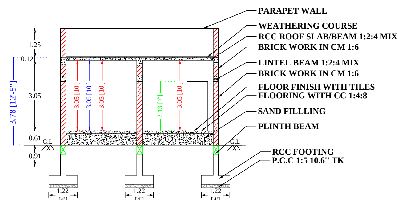
SECTION - "AA"
