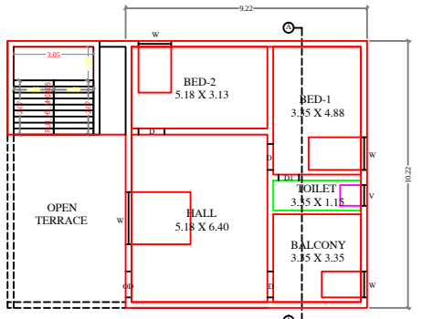
FLOOR-1
