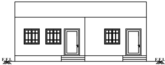
ELEVATION FACING ON EAST
