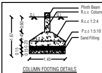
COLUMN FOOTING DETAILS
