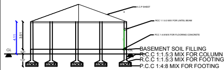
SECTION ON A-A
