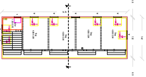
Proposed Scale:- 1:100 PROPOSED GROUND FLOOR
