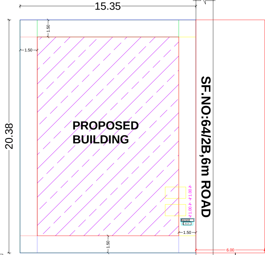
SITE PLAN
