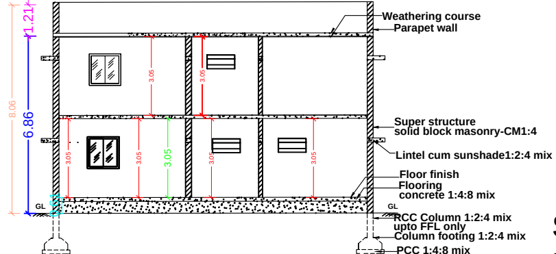
SECTION ELEVATION
