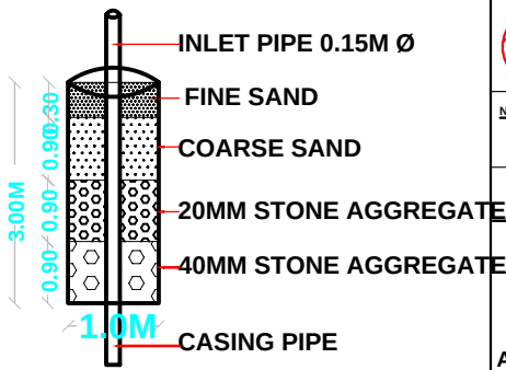
DETAILS OF RAIN WATER
