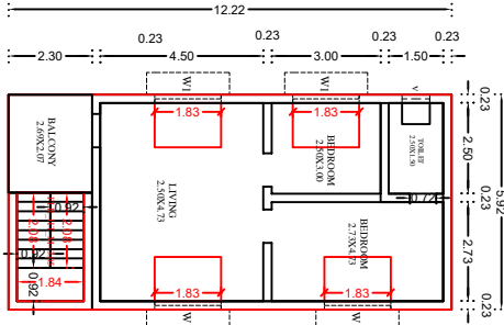
PRO. FIRST FLOOR PLAN
