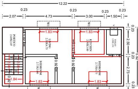
PRO. GROUND FLOOR PLAN
