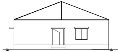
EAST SIDE ELEVATION
