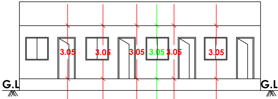
ELEVATION FACING ON NORTH
