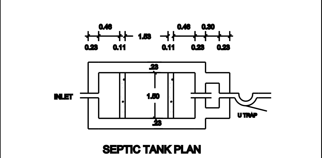
SEPTIC TANK PLAN
