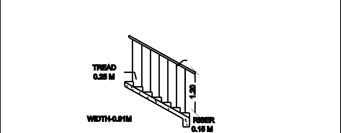
STAIRCASE DETAILS
