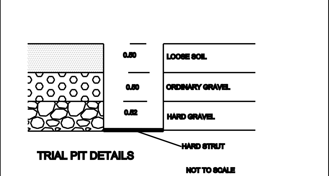
TRIAL PIT DETAILS
