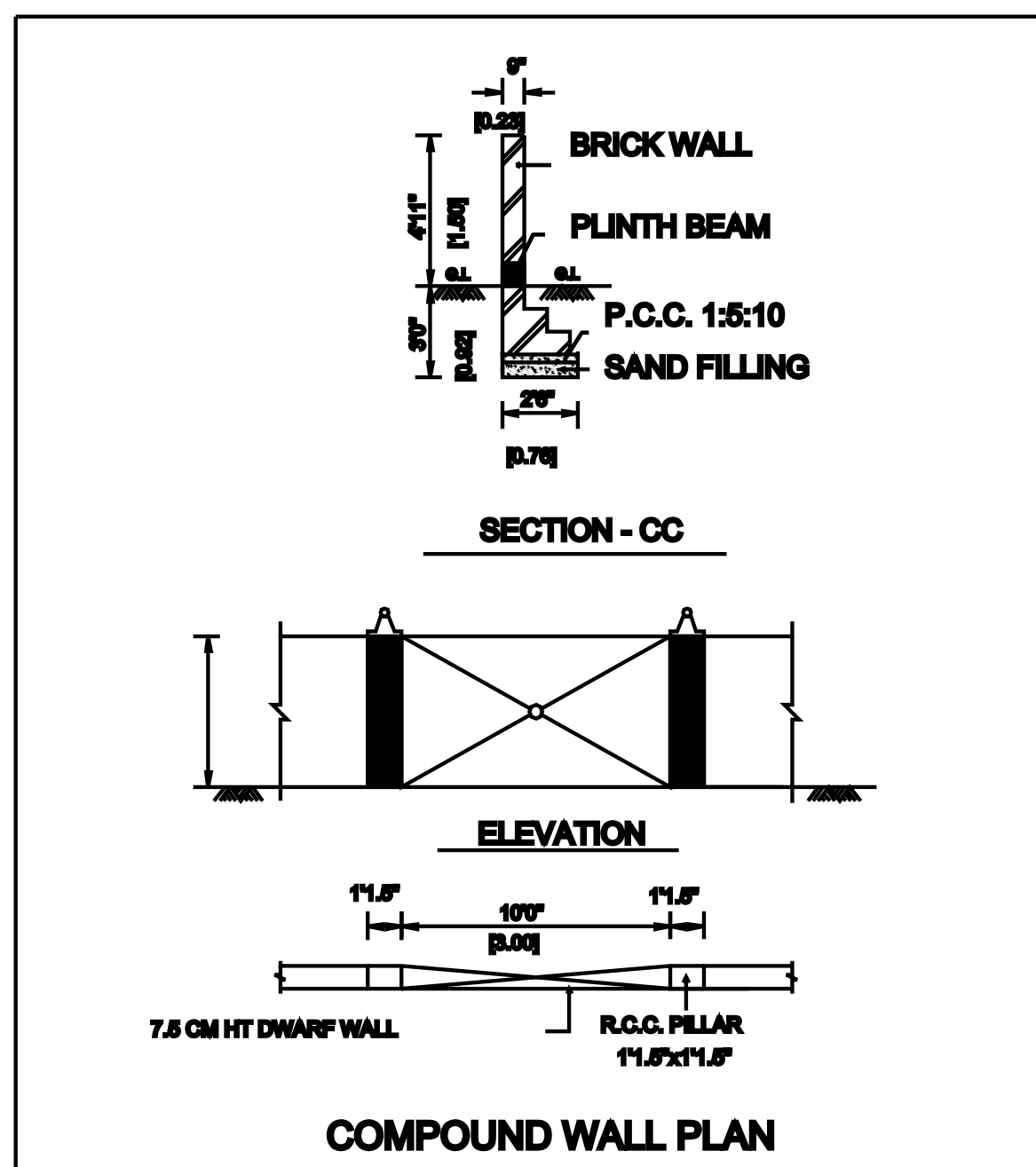
COMPOUND WALL PLAN
