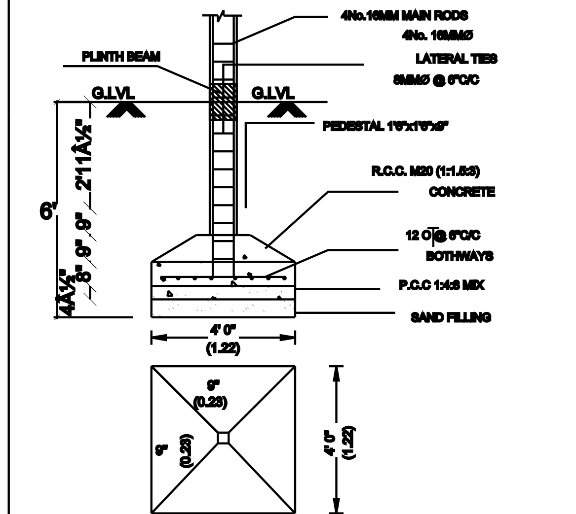
FOUNDATION DETAIL
