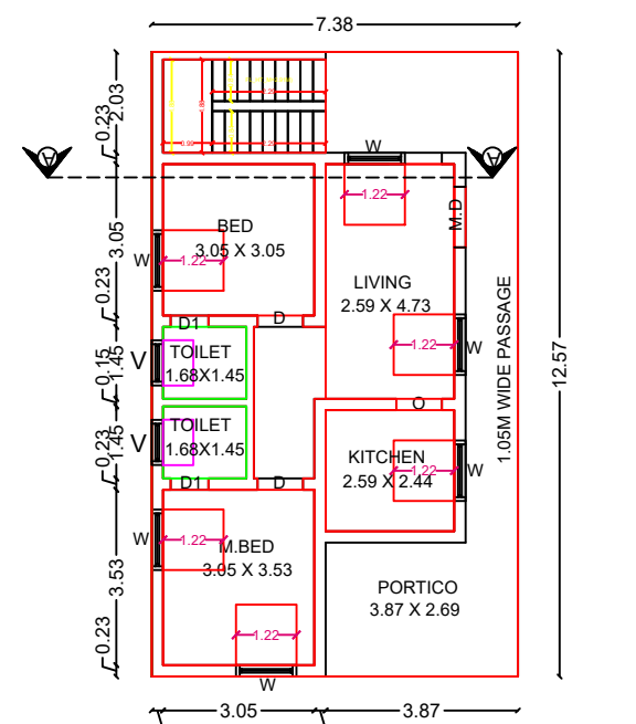
PRO. GROUND FLOOR (G.F) PLAN
