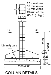
COLUMN DETAILS
