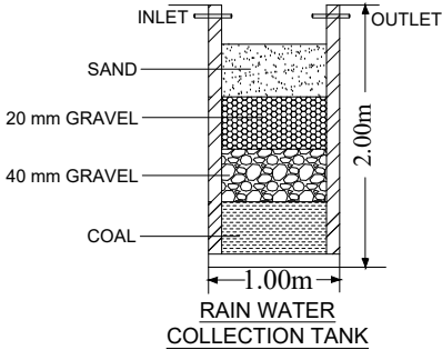
RAIN WATER COLLECTION TANK
