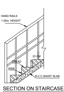
SECTION ON STAIRCASE
