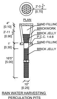
RAIN WATER HARVESTING PERCOLATION PITS
