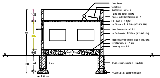
Section on "BC"
