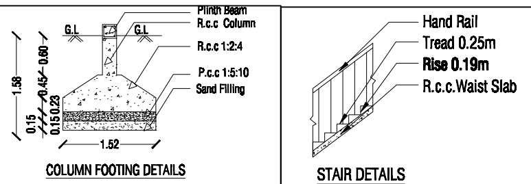
COLUMN FOOTING DETAILS
