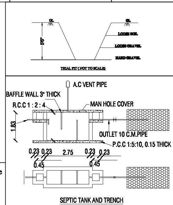
SEPTIC TANK AND TRENCH
