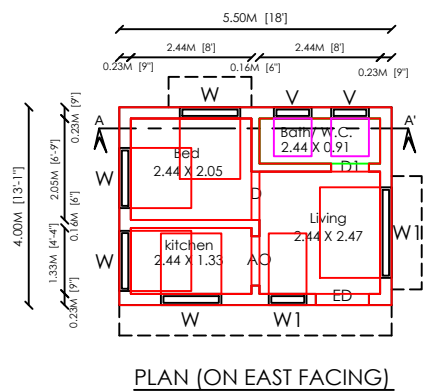
PLAN (ON EAST FACING)
