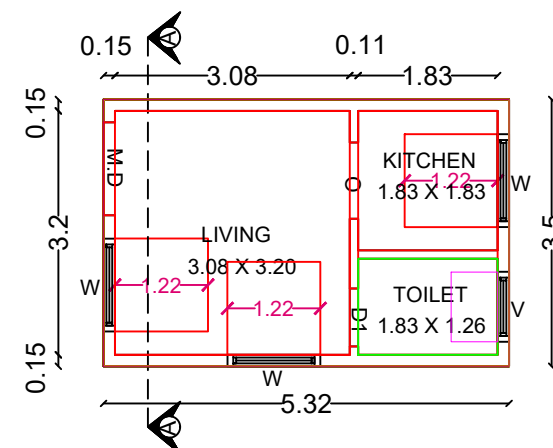
PRO.GROUND FLOOR (G.F) PLAN
