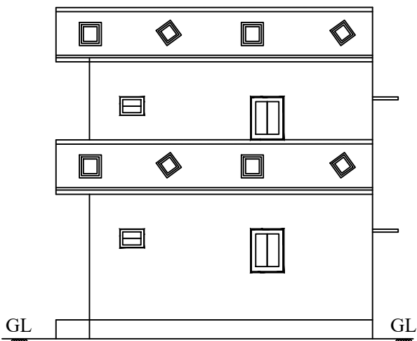
ELEVATION ON WEST FACE
