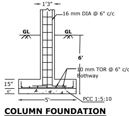
COLUMN FOUNDATION
