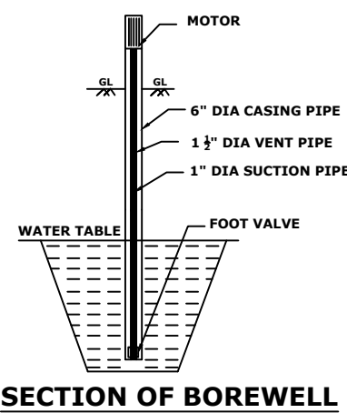
SECTION OF BOREWELL
