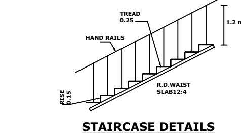
STAIRCASE DETAILS
