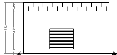
ELEVATION FACING EAST
