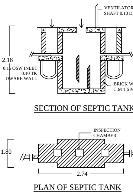
SEPTIC TANK
