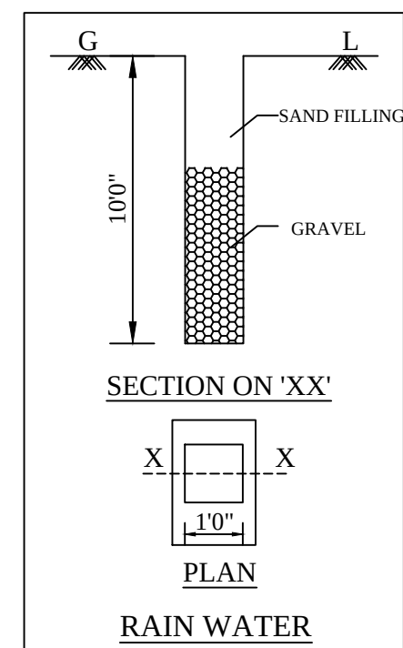
RAINWATER HARVESTING
