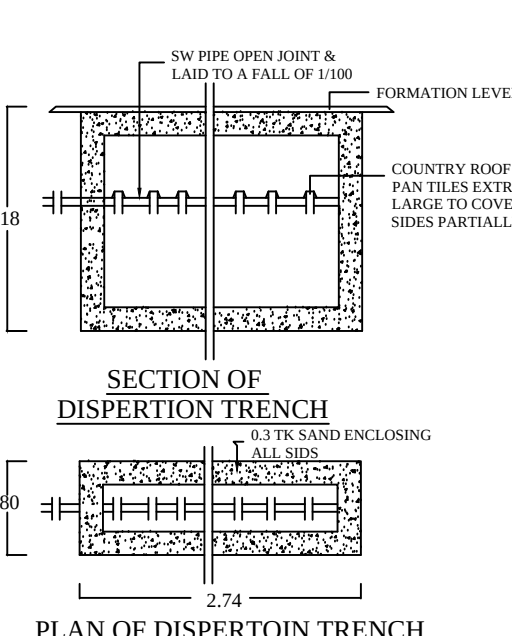
DISPERSION TRENCH
