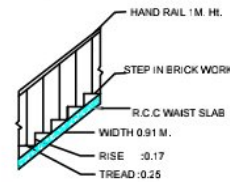
STAIR DETAIL
