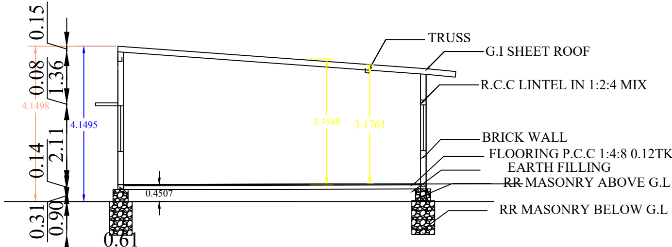
CROSS SECTION ON 'AB'
