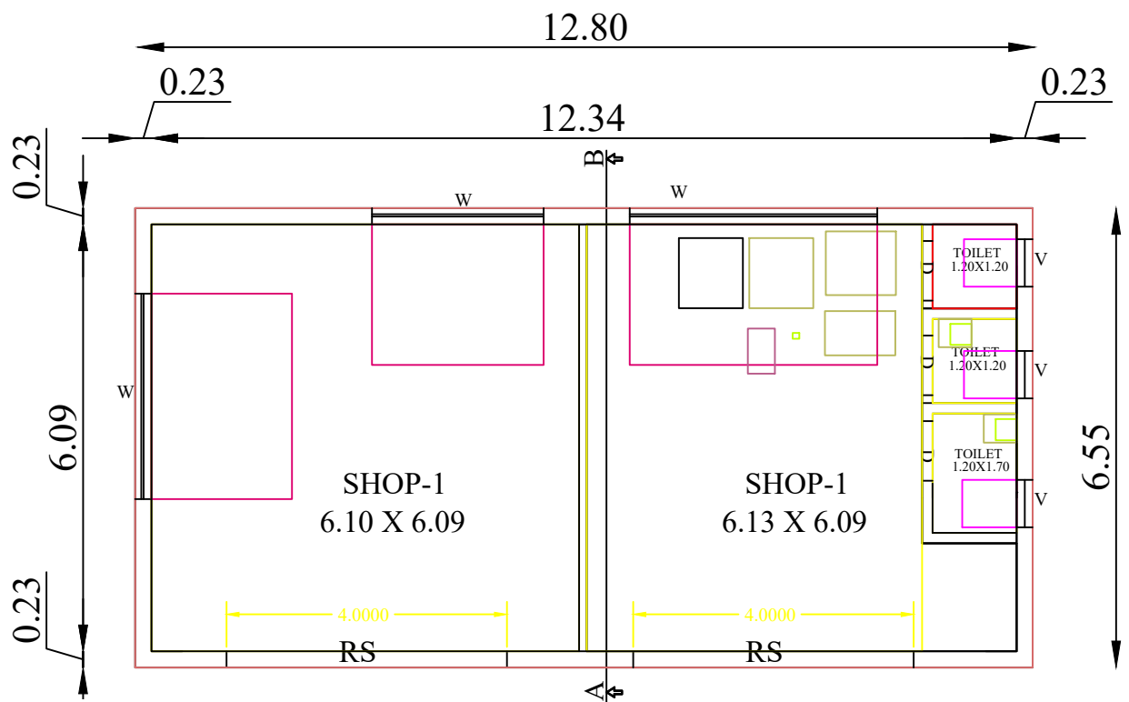
FLOOR PLAN
