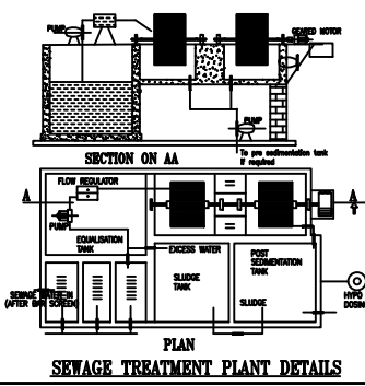
SEWAGE TREATMENT PLANT DETAILS
