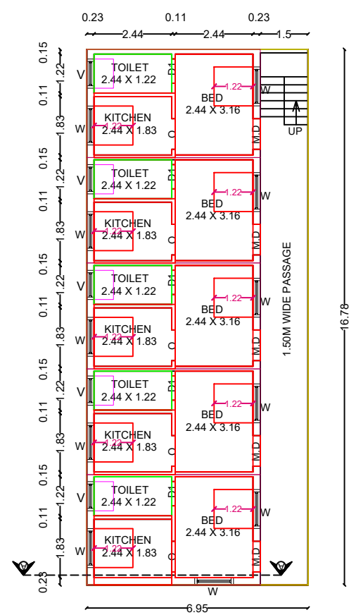
PRO.GROUND FLOOR (G.F) PLAN
