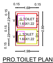
PRO.TOILET PLAN
