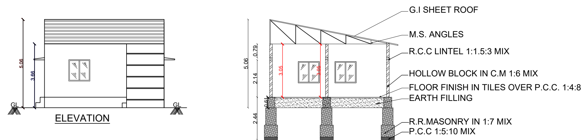
SECTION "A-A"
