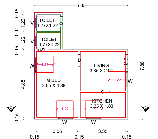
PRO.GROUND FLOOR (G.F) PLAN
